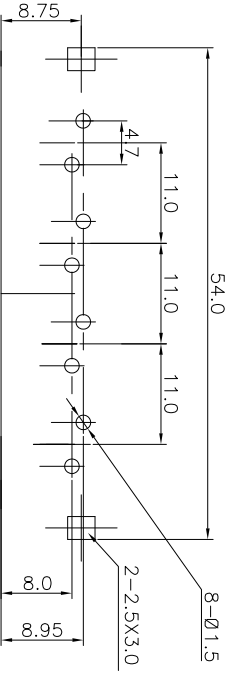
PCB LAYOUT TOP VIEW
