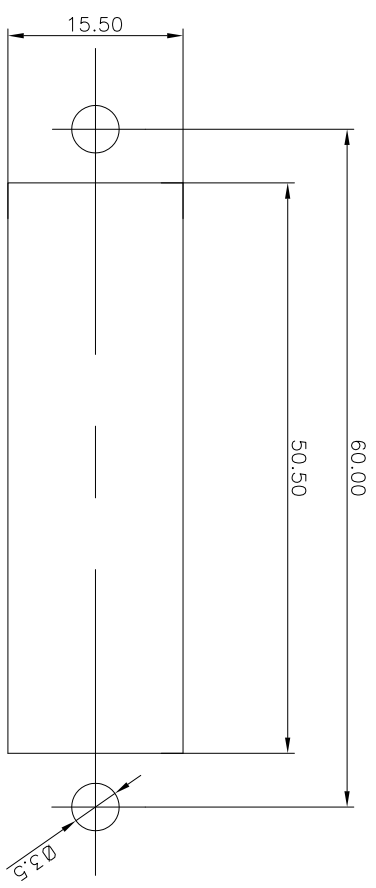
PANEL CUTOUT
