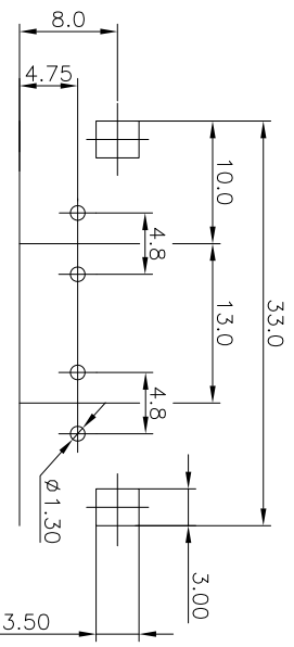
PCB LAYOUT TOP VIEW
