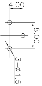
PCB LAYOUT TOP VIEW
