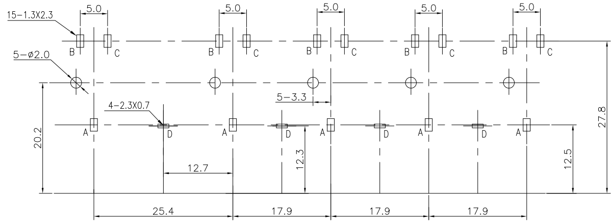
PCB LAYOUT TOP VIEW
