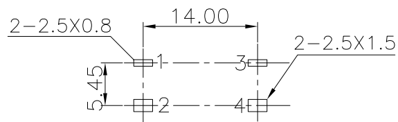
PCB LAYOUT TOP VIEW
